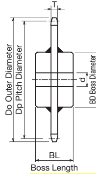
C-Type Welded Specification
